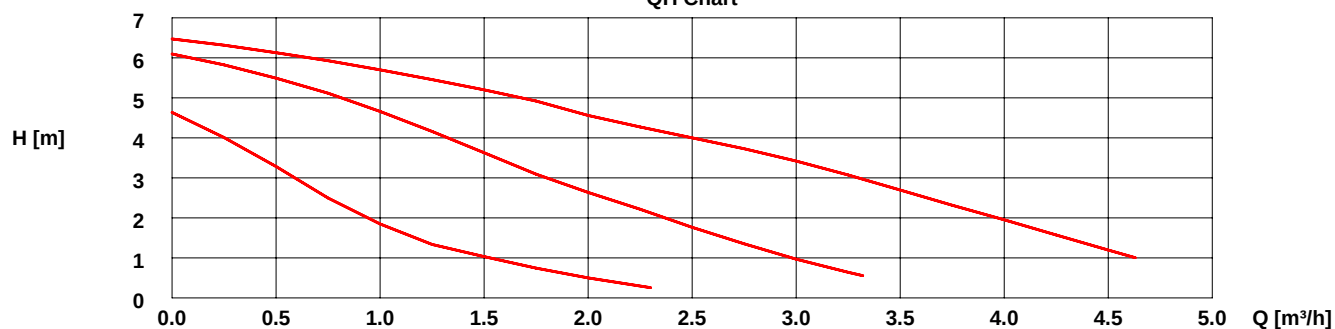
QH Chart
