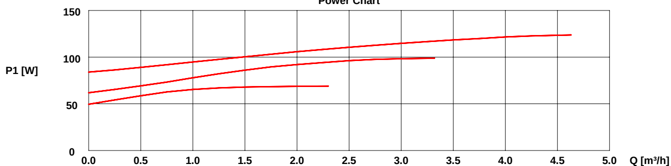
Power Chart
