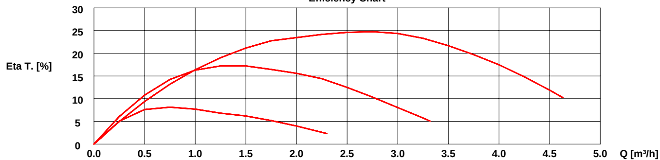
Efficiency Chart
